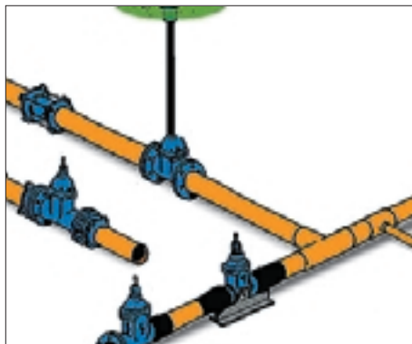
Gas below ground
